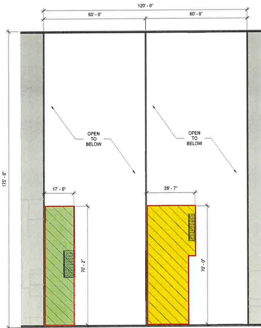
1 Premises Diagram - 2nd Floor
